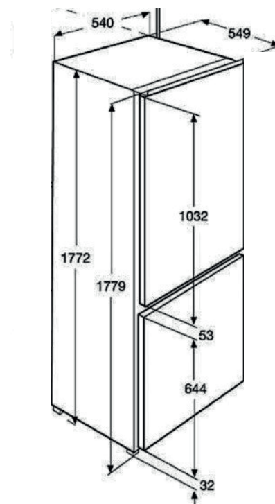
Whirlpool ART 7811 Whirlpool ART 895/A++NE Whirlpool ART 65021 (schemat)
