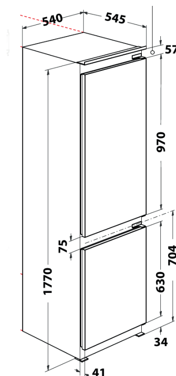
Whirlpool ART 7811 Whirlpool ART 895/A++NE Whirlpool ART 65021 (schemat)
