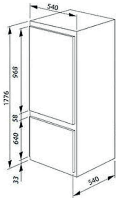
Amica BK3265-4U Amica BK3165.4AA (schemat)
